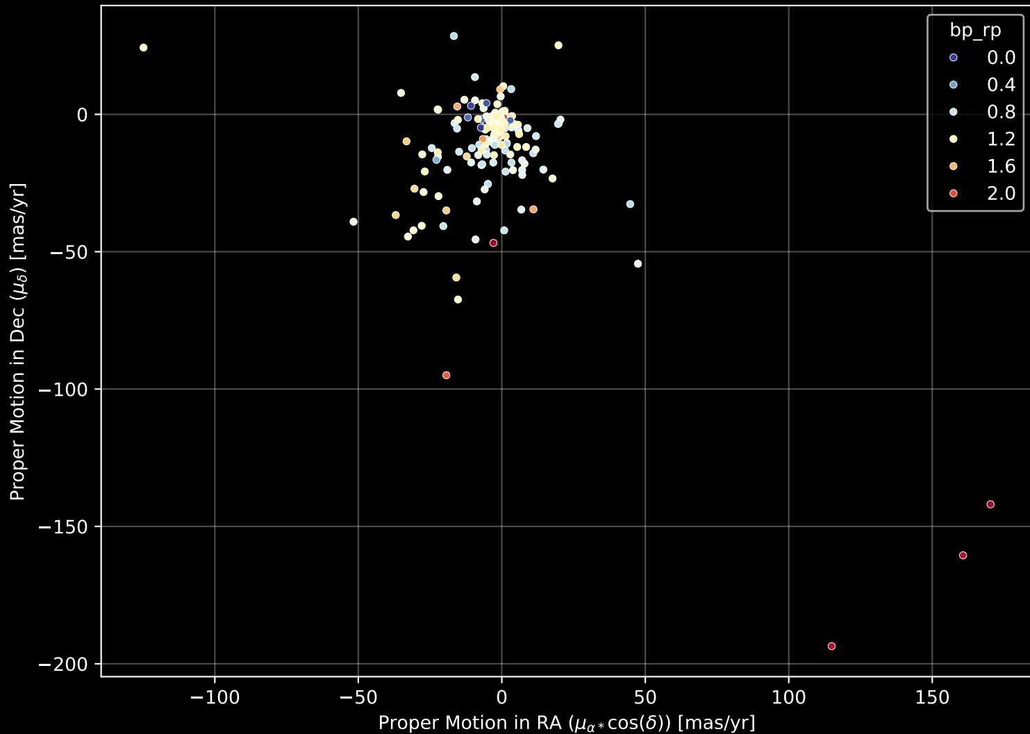
APOGEE DR17 Field: [198+21_MGA] Proper Motion Diagram (n= 192)
