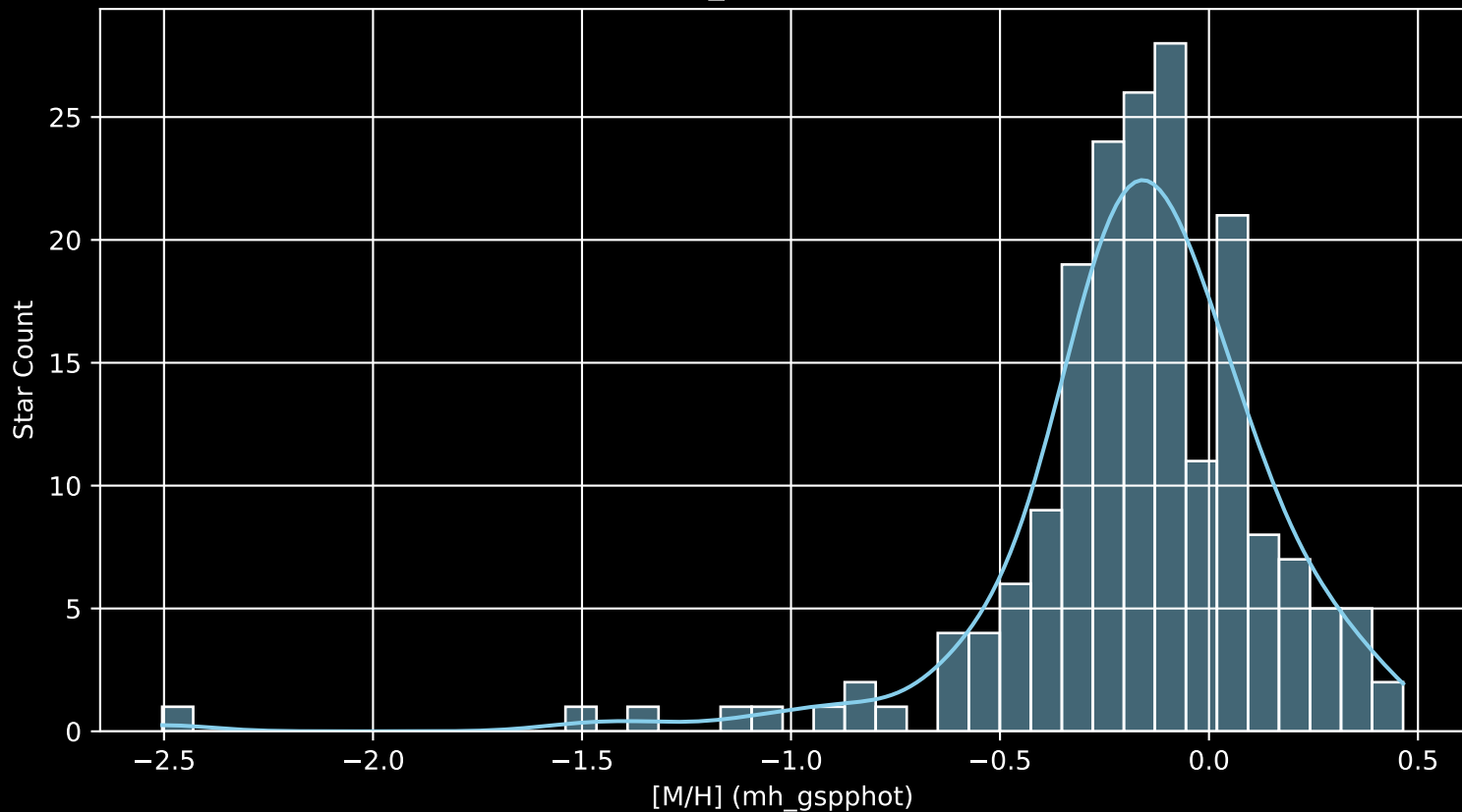
APOGEE DR17 Field: [198+21_MGA [M/H] (mh_gspphot) (n= 188)
