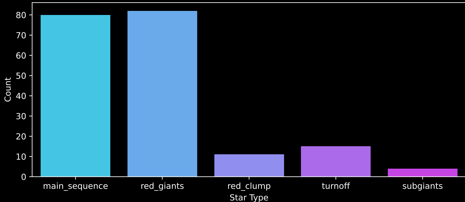
APOGEE DR17 Field: [198+21_MGA] Count plot of Star Type
