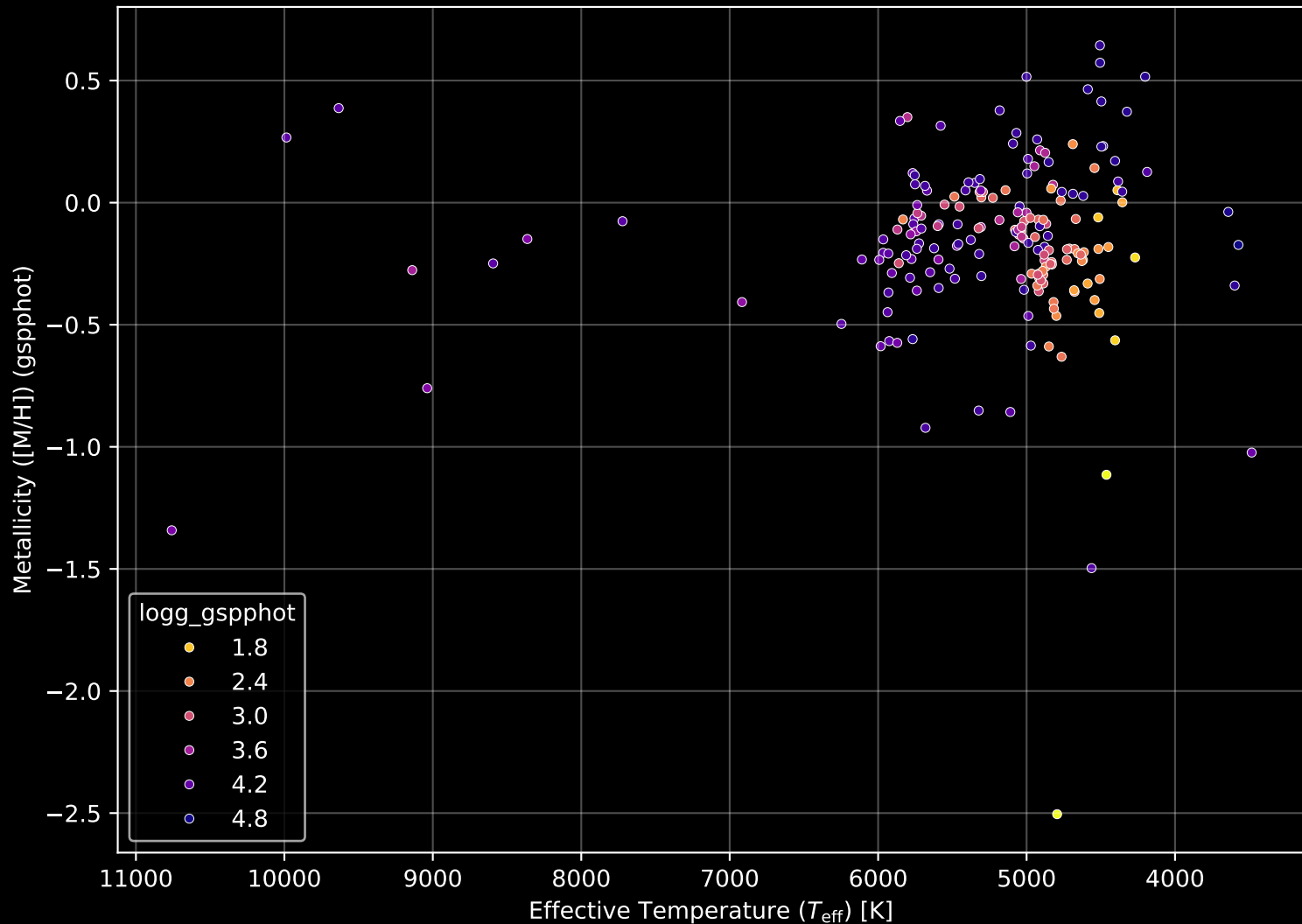
APOGEE DR17 Field: [198+21_MGA] Stellar Population Parameters (n= 192)
