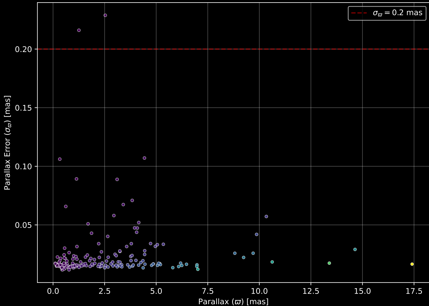
APOGEE DR17 Field: [198+21_MGA] Parallax Quality (n= 192)
