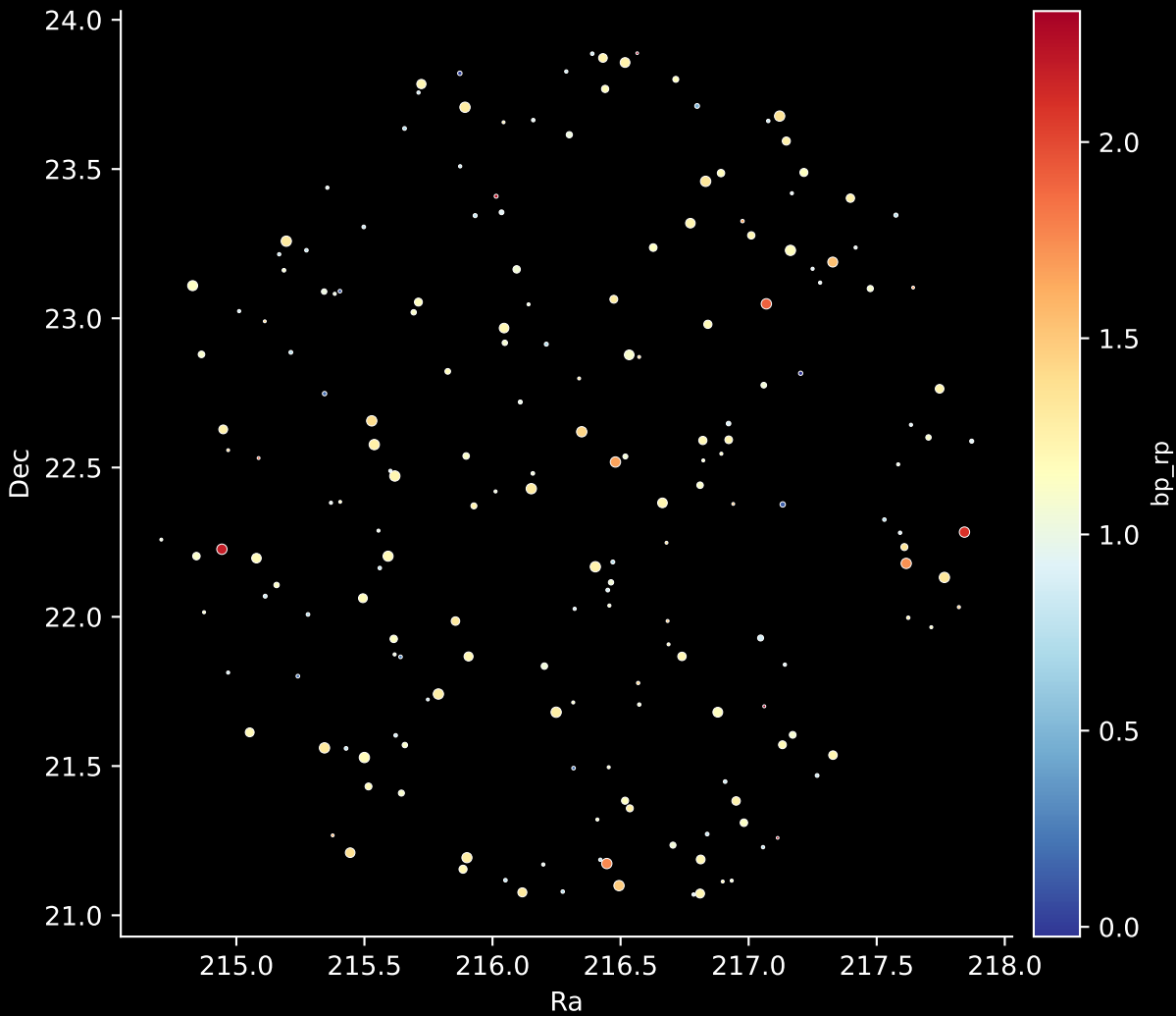
APOGEE DR17 Field: [198+21_MGA] Stars: 192
