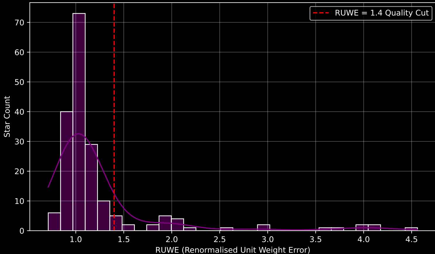
GAPOGEE DR17 Field [198+21_MGA] RUWE Distribution (n= 187)
